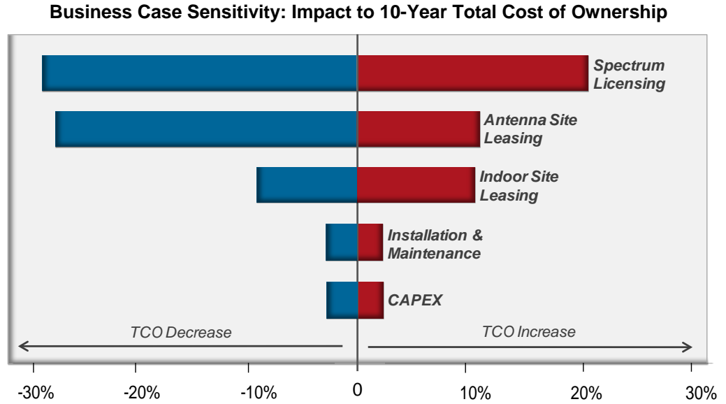
Figure 2: Backhaul business case variables and their potential range of impact to TCO. 4
