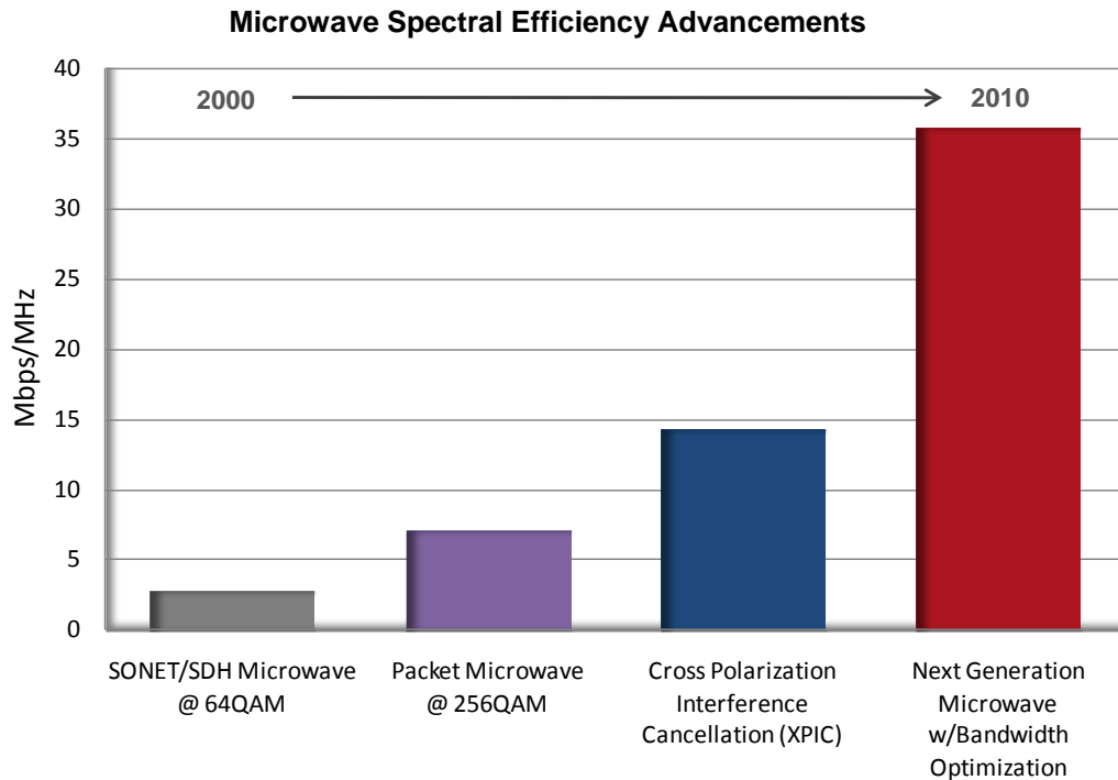
Figure 4: Spectral efficiency improvements through each generation of microwave. 5
