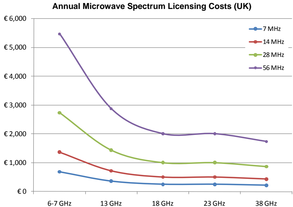
Figure 1: Annual spectrum licensing cost per link. 2
